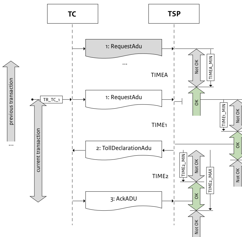
Sequence diagram of the TOLLDECLARATION transaction from EN 16986:2024.
