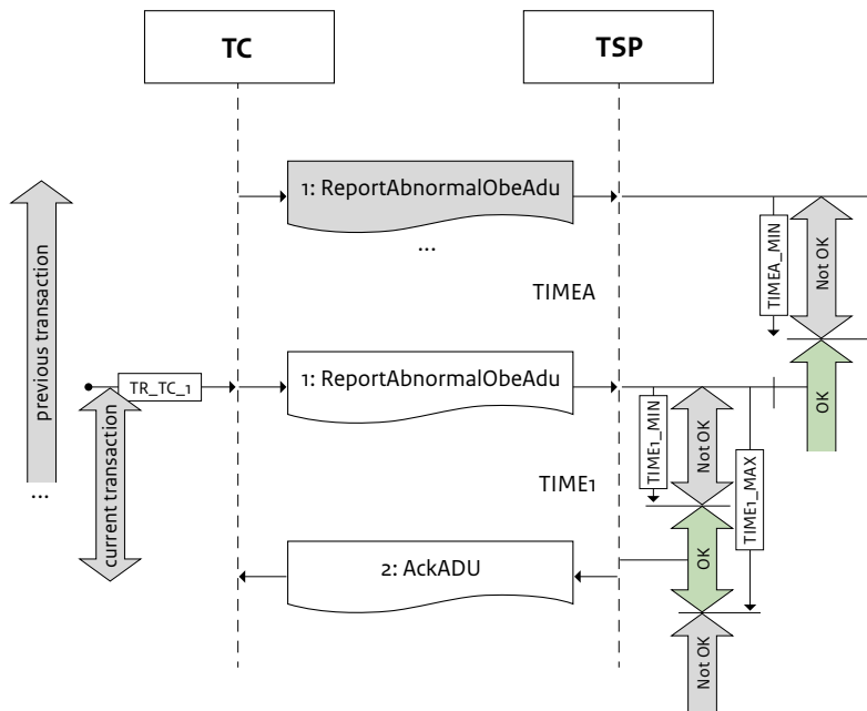
Sequence diagram of the REPORTABNORMALLOBE transaction from EN 16986:2024.
